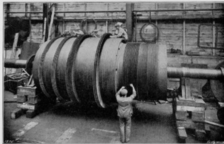
Fig. 21. Blading a Rotor at the Turbina Works.
