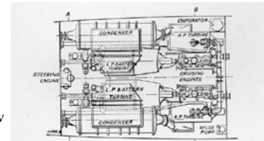
Fig. 41. First set of Combination Machinery—in H.M.S. "Velox."
