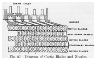
Fig. 27. Diagram of Curtis Blades and Nozzles.
