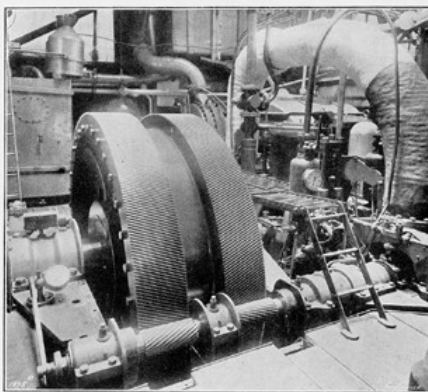
Fig. 49. View of Gearing in "Vespasian."
