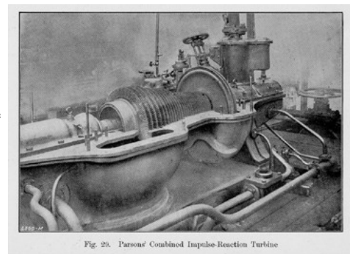
Fig. 29. Parsons' Combined Impulse-Reaction Turbine
