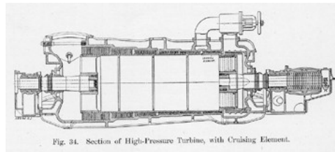
Fig. 34. Section of High-Pressure Turbine, with Cruising Element.
